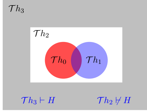
Figure 2. Map (territories) of four theories w.r.t. their sets of theorems
